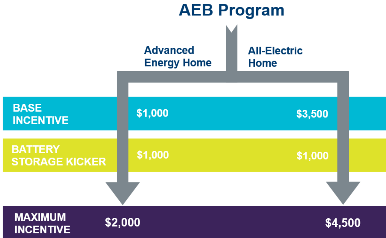
Figure 2. Pathway Graphic
