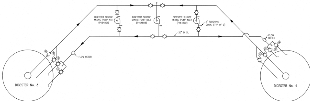
Figure 10-3: Externally Pumped Mixing System Schematic
