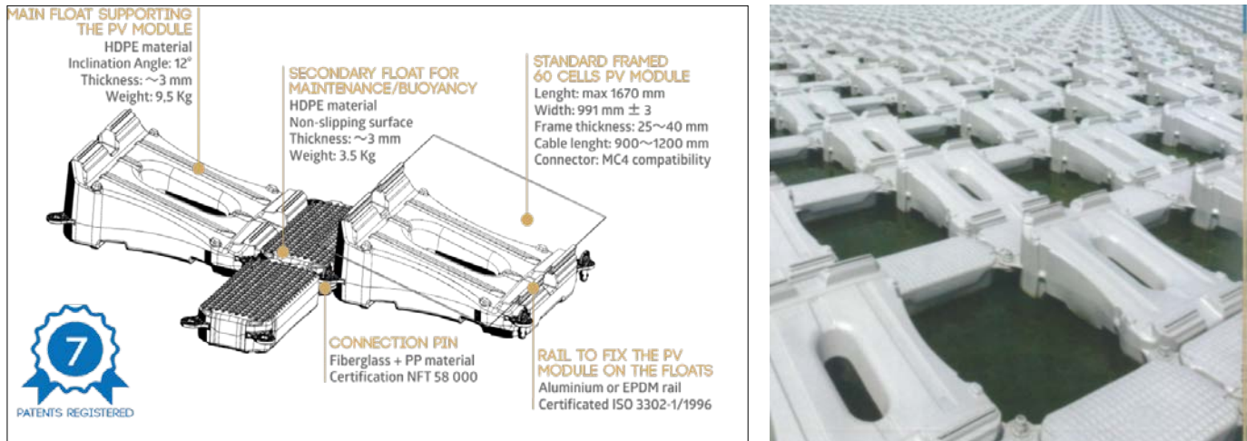
Figure B-4: Ciel & Terre's Hydrelío Modular System
